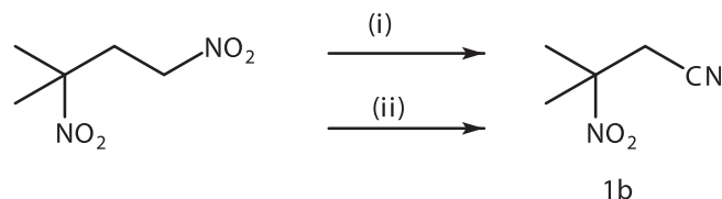
Scheme 3. Reduction of 3-methyl-1,3-dinitrobutane to 3-methyl-3-nitrobutanenitrile ( 1b ), (i): NaBH 2 S 3 /THF, reflux, 5 h, 62%, (ii): PCl 3 /pyridine, rt, two days, 81%.
