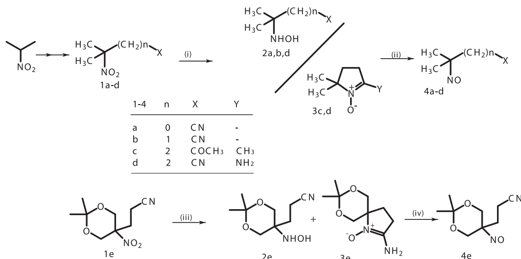
Scheme 2. Synthesis of the target nitroso compounds 4 from the corresponding nitro compounds 1 ; (i): Al/Hg, Et 2 O/H 2 O, rt, 18–85%; (ii): Cl 2 /H 2 O, 0 °C or MCPBA/CHCl 3 , 0 °C or NaO 4 /H 2 O, rt, 21–92%, (iii): Al/Hg, THF/H 2 O, rt, 92%, (iv): NaO 4 /H 2 O, rt, 77%.
