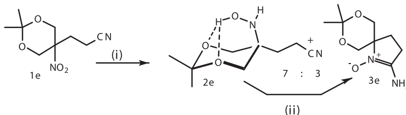
Scheme 4. Reduction of 5-(2-cyanoethyl)-2,2-dimethyl-5-nitro-1,3-dioxane ( 1e ) affording hydroxylamine 2e and nitronone 3e (7:3 mol/mol), (i): Al(Hg), THF/H 2 O, rt, 2 h, 92%; (ii): TMG/THF, reflux, 5 h.
